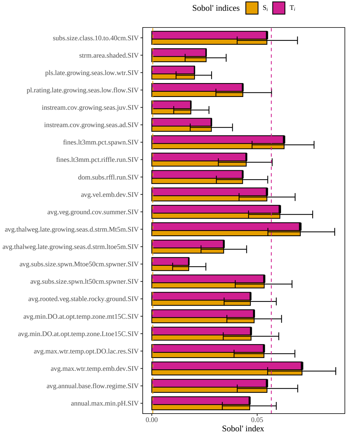
Figure 4. Results of a sensitivity analysis for the rainbowtroutRiv model based on an arithmetic mean structure. Dashed lines represent baseline numerical approximation error for S_i and T_i ( i.e. , dummy variables).
